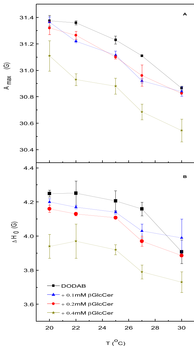
Fig. 4. Effect of \beta GlcCer on the maximum hyperfine splitting ( A_{max} ) of 5-PCSL (A) and on the central field linewidth ( \Delta H_0 ) of 16-PCSL (B) embedded in 2 mM DODAB bilayers at the gel phase.
