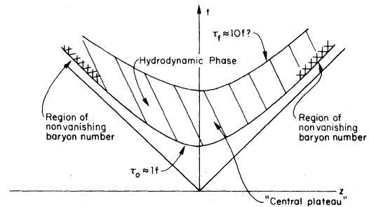
FIG. 3. Space-time diagram of longitudinal evolution of the quark-gluon plasma.
