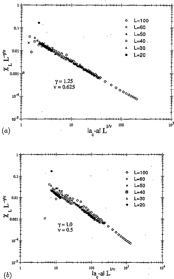
Figure 7. (a) Plot of \chi_L L^{-\gamma/\nu} against (a_c - a)L^{1/\nu} along the line y = 1 . (b) Plot of \chi_L L^{-\gamma/\nu} against (a_c - a)L^{1/\nu} along the line y = 2x .
