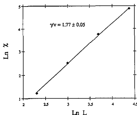
Figure 6. Log-log plot of X_L at the critical point against L for the case x = 1 .
